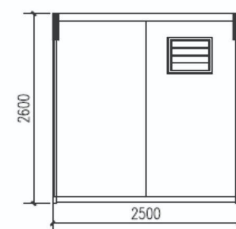
Back elevation
